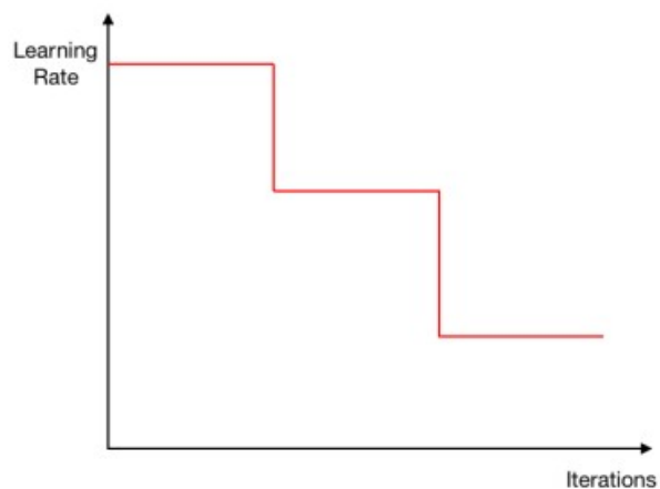
梯级衰减 (step decay)
